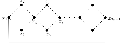
Fig. 5. An equality formula corresponding to the crafted examples.
