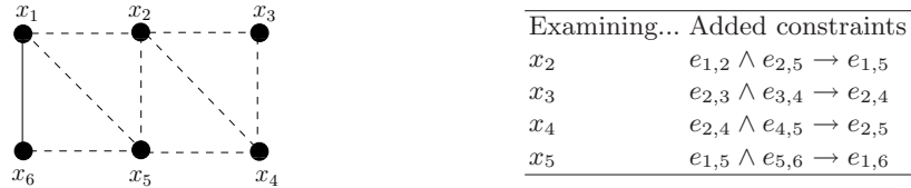
Fig. 3. An Equality Graph for Example 3.
