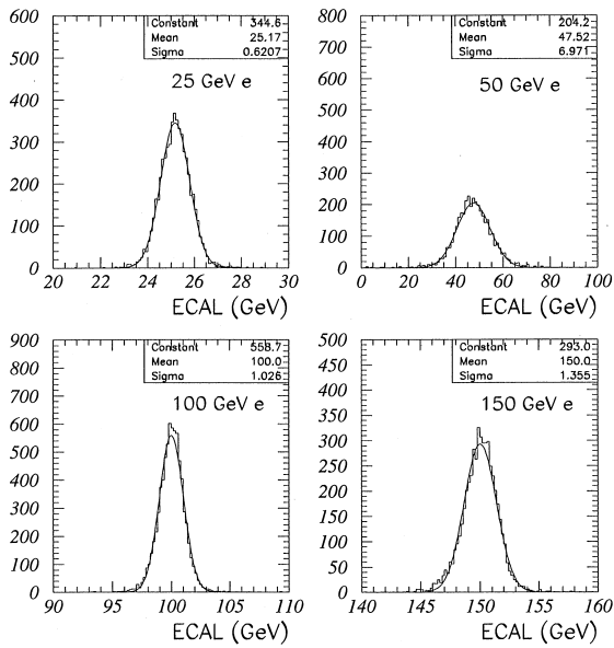
Fig. 22. H4(1995) data: response of the \text{PbWO}_4 crystal ECAL calorimeter to 25,50,100 and 150 GeV/c electrons.
