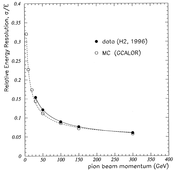
Fig. 38. H2(1996), B = 0 T data: the fractional energy resolution of the hadron calorimeter (HCAL only) for pions and comparison with the GEANT-GCALOR MC simulation. The electromagnetic calorimeter has been taken out of the beamline.
