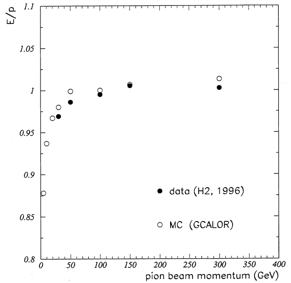
Fig. 37. H2(1996), B = 0 T data: linearity of the energy response of the hadron calorimeter (HCAL only) for pions and comparison with the GEANT-GCALOR MC simulation. The electromagnetic calorimeter has been taken out of the beamline.
