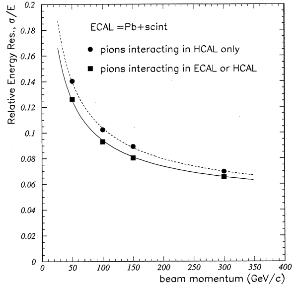
Fig. 21. H2(1995) data: fractional energy resolutions for “mip-in-ECAL” pions and “full pion sample”. The statistical errors are smaller than the size of the symbols.
