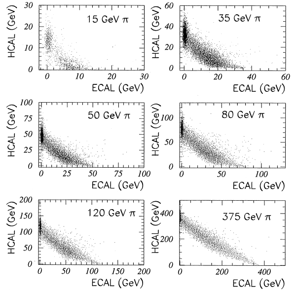
Fig. 23. H4(1995) data: scatter plots of the energy in HCAL versus the energy in the \text{PbWO}_4 crystal ECAL calorimeter for pions.
