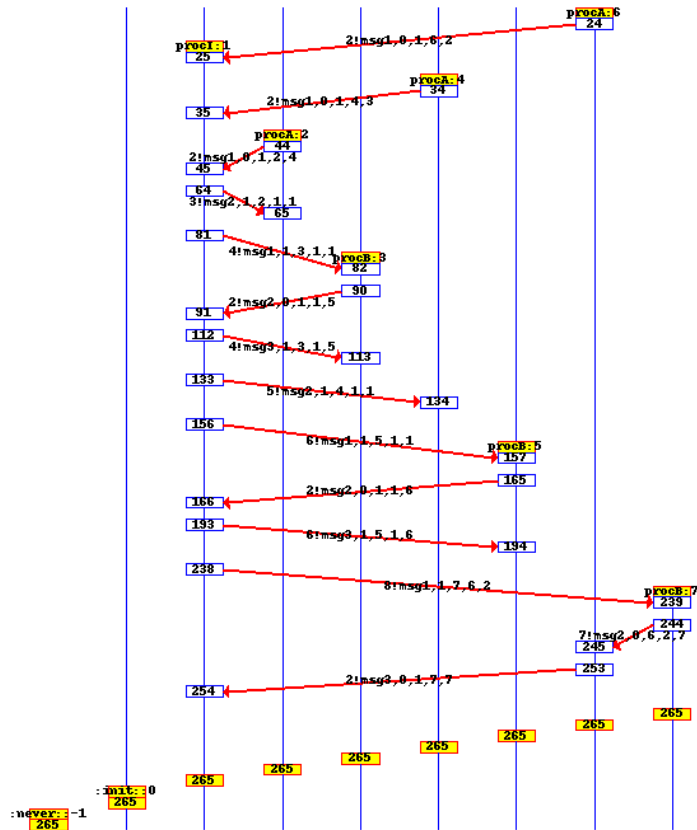
Figure 4: Lowe's attack with 6 processes
