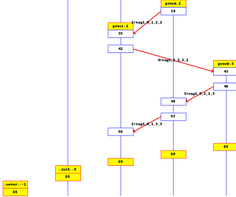
Figure 3: Lowe’s attack on the Needham-Schroeder protocol, discovered by SPIN
