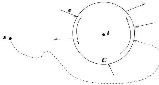
Figure 9. t inside cycle C , s outside
