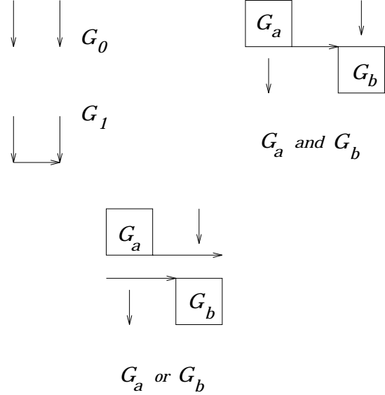
Figure 8. The construction of G_\phi . All south edges are present.
