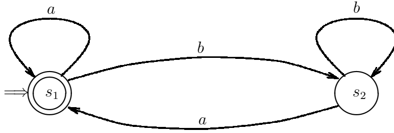
Figure 2: A Büchi automaton for L (Example 1.1)
