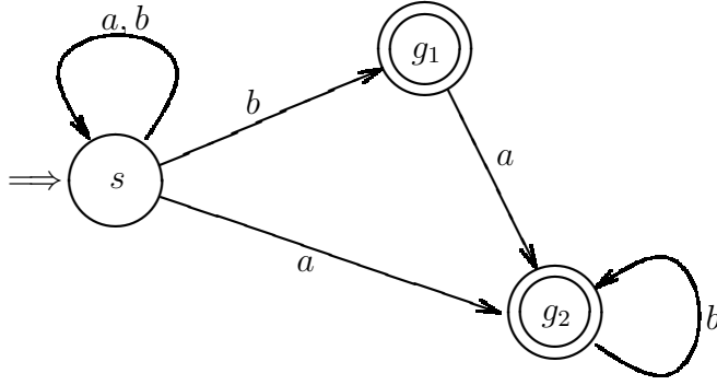
Figure 9: The hierarchical marked subset construction is not sound (Example 4.5)
