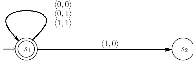
Figure 4: Büchi automaton for the atomic formula X \subseteq Y
