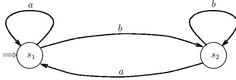
Figure 6: Automaton for L and \overline{L} (Example 3.1)
