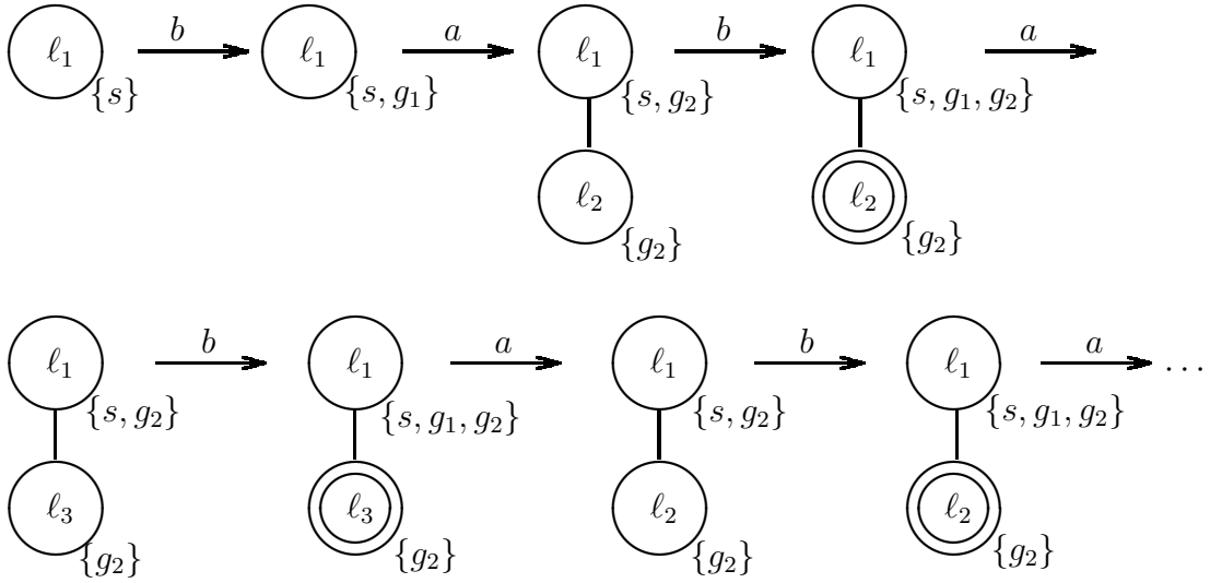
Figure 10: A run generated by Safra's construction
