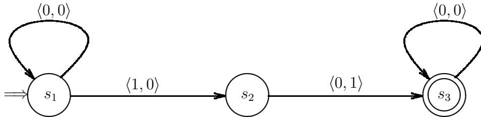
Figure 5: Büchi automaton for the atomic formula \text{succ}(X, Y)
