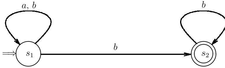
Figure 3: A Büchi automaton for \bar{L} (Example 1.1)
