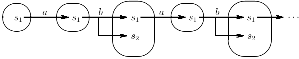
Figure 7: A run of the extended subset automaton for \overline{L} on input (ab)^\omega (Example 4.1)
