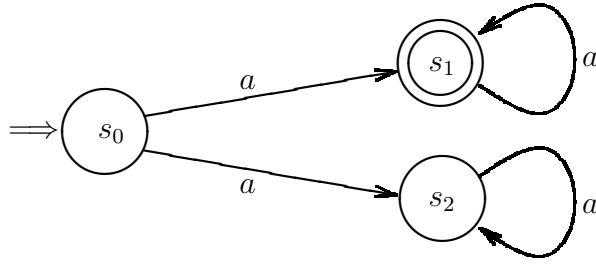
Figure 8: The marked subset construction is not complete (Example 4.3)
